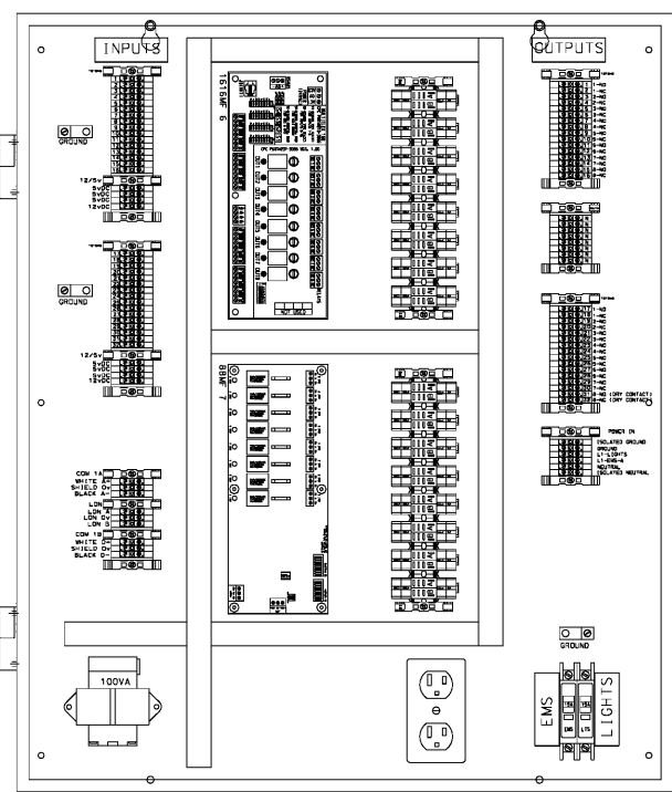
EMS A INTERIOR ELEVATION
