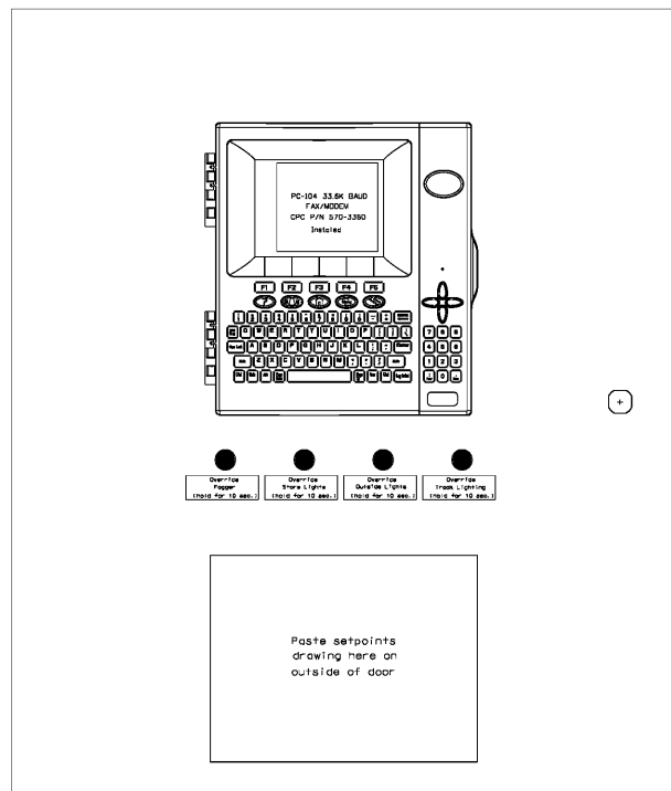
EMS A EXTERIOR ELEVATION
