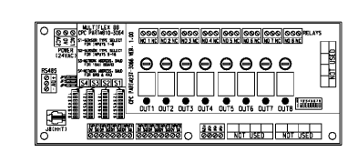
TYP. MULTIFLEX 88 I/O BOARD AT A/C UNIT
