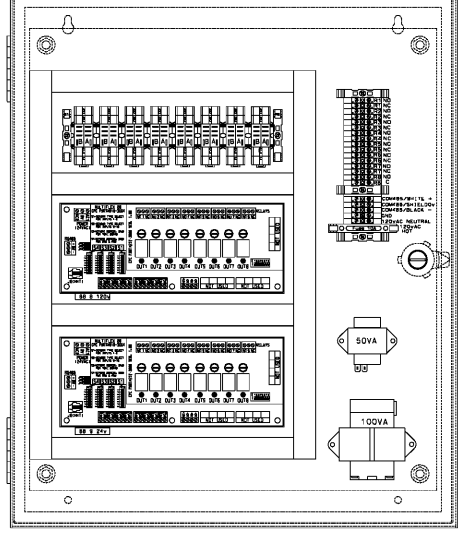
EMS B & D INTERIOR ELEVATION
