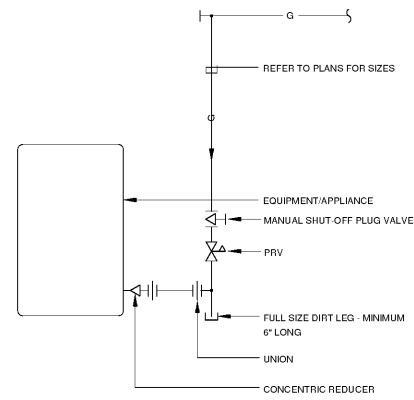
2 DETAIL - GAS EQUIPMENT CONNECTION SCALE: N.T.S.
