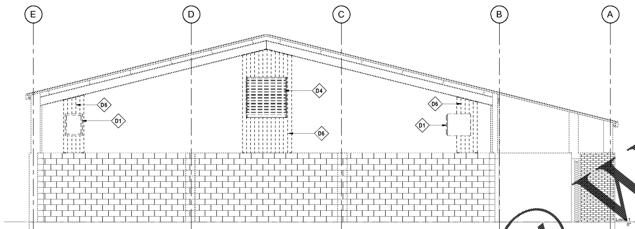
3 DEMOLITION SECTION 1/4" = 1'-0"
