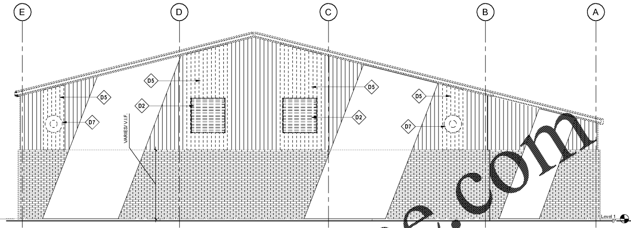
2 DEMOLITION SOUTH ELEVATION 1/4" = 1'-0"
