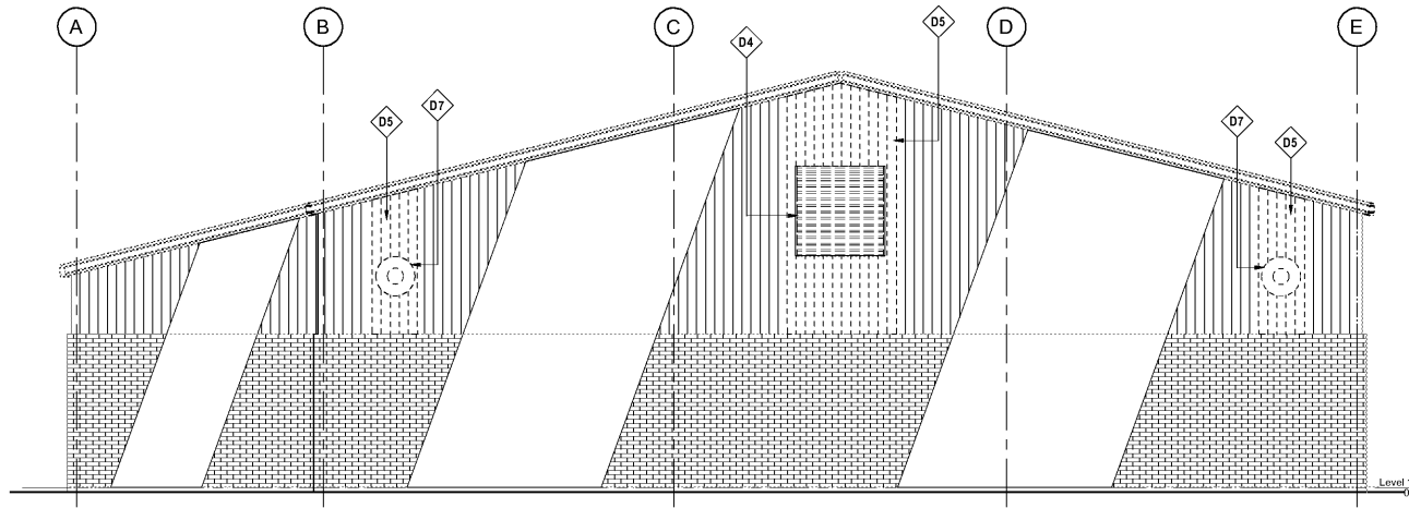
1 DEMOLITION NORTH ELEVATION 1/4" = 1'-0"
