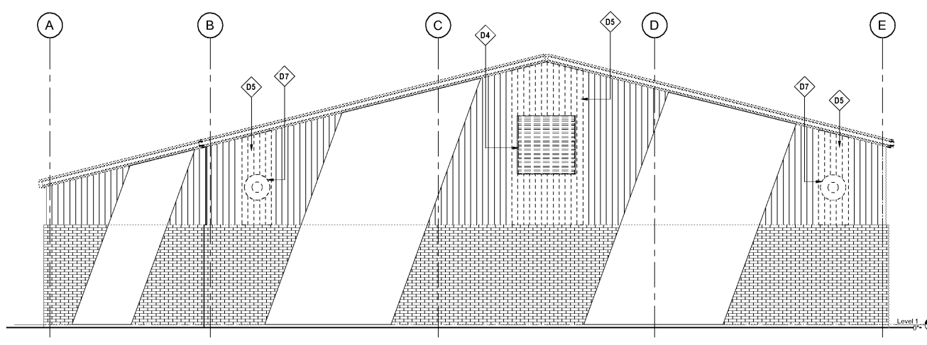
1 DEMOLITION WEST ELEVATION 1/4" = 1'-0"
