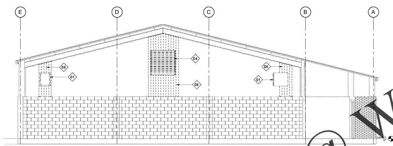
3 DEMOLITION SECTION 3 1/4" = 1'-0"
