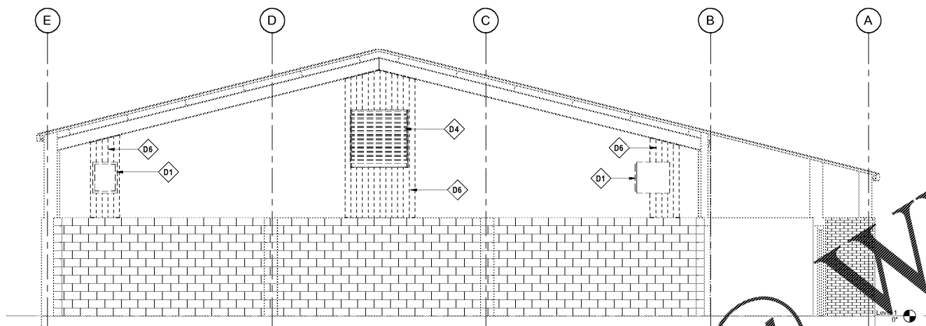
3 DEMOLITION SECTION 3 1/4" = 1'-0"
