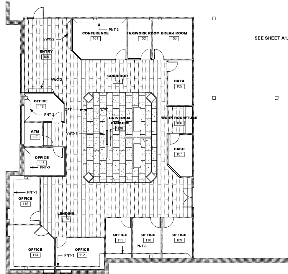
1 1ST FLOOR FINISH PLAN SCALE: 1/8" = 1'-0"
