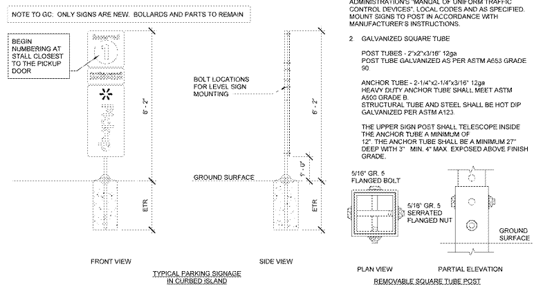
1 PARKING SIGN MOUNTING AND BASE 1/2" = 1'-0"
