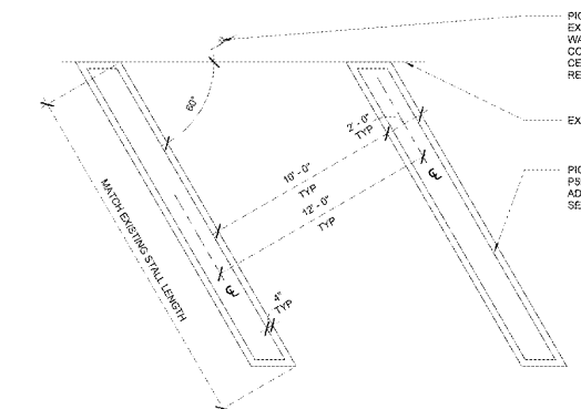
2 PICKUP PARKING STALL DETAIL 1/4" = 1'-0"
