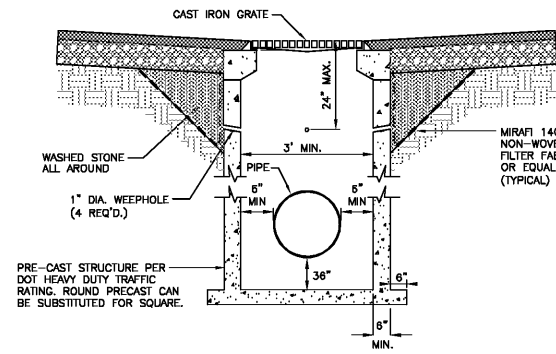
CATCH BASIN/JUNCTION BOX N.T.S.
