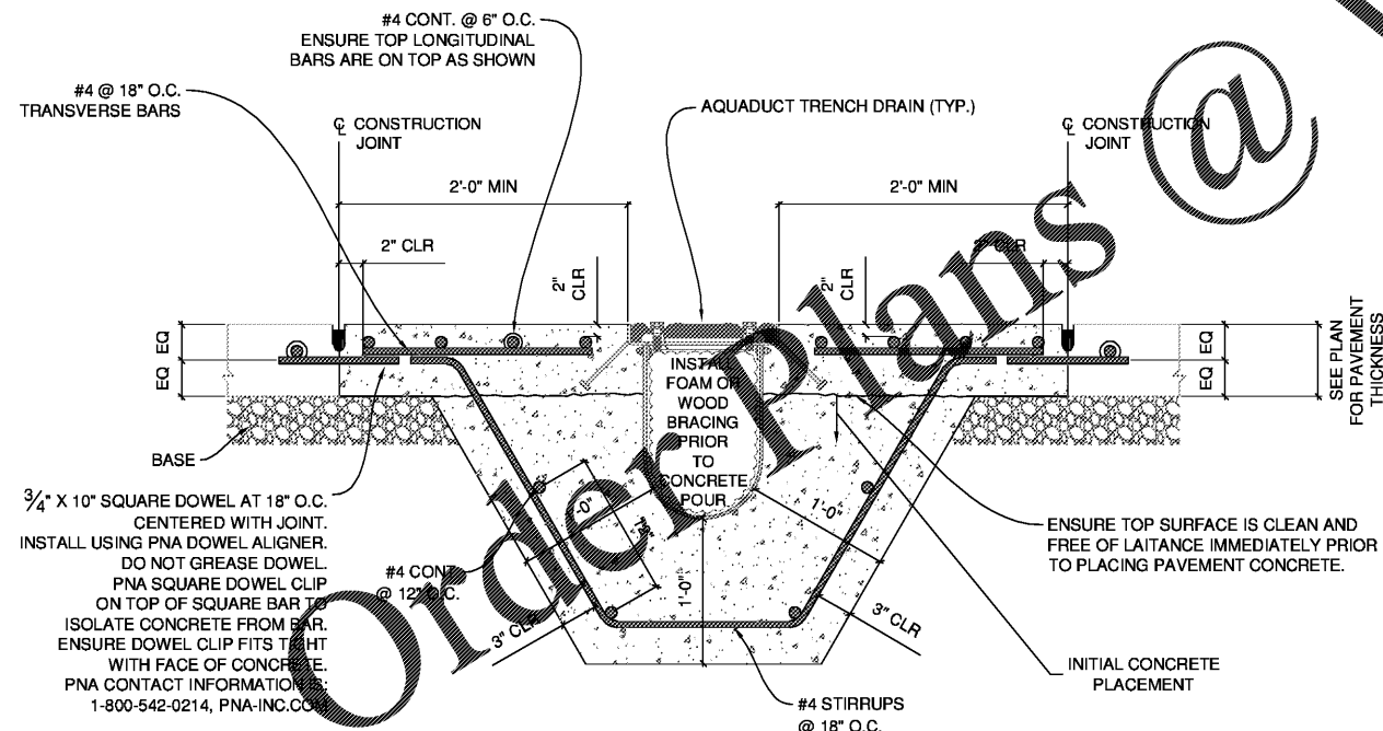
TYP. CONCRETE AQUADUCT TRENCH DRAIN DETAIL N.T.S.
