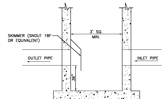
STORM STRUCTURE SUMP W/ SKIMMER N.T.S.
