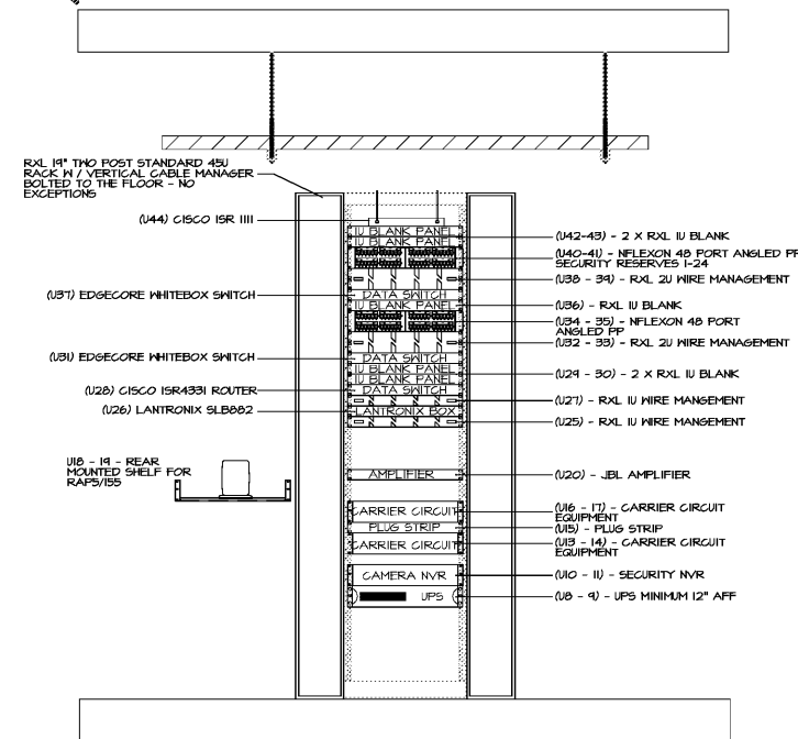
5 TELCO RACK ELEVATION SCALE: NONE
