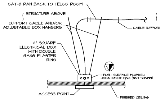
2 CEILING MOUNT ACCESS POINT DETAIL SCALE: NONE (SYMBOL)
