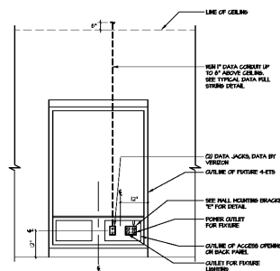
3 POWER DIAGRAM FOR 4-ETS N.T.S.
