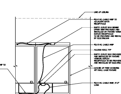
4 POWER DIAGRAM FOR FREE STANDING 4FT CABINETS N.T.S.
