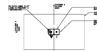
18 FLOOR BOX LOCATION DIAGRAM FOR 4-POS N.T.S.
