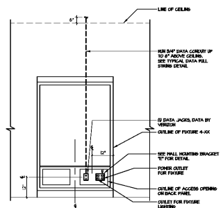
2 POWER DIAGRAM FOR 4-XX N.T.S.
