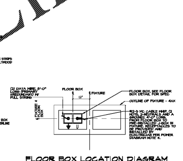
10 FLOOR BOX LOCATION DIAGRAM FOR FREESTANDING 4-XX FOR FIXTURES: 4-SK, 4-SS, 4-SK, 4-SS N.T.S.
