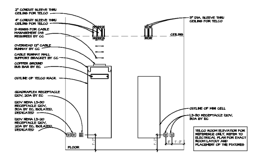
7 TYPICAL TELCO RACK AND MINI CELL (WHERE APPLICABLE) ELEVATION N.T.S.
