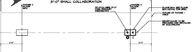
17 FLOOR BOX LOCATION DIAGRAM FOR COLLAB AND EXP. TABLES N.T.S.
