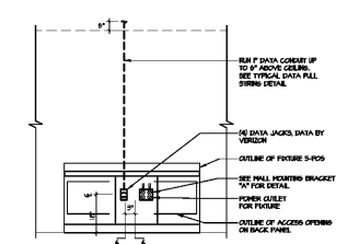
6 POWER DIAGRAM FOR 3-POS N.T.S.
