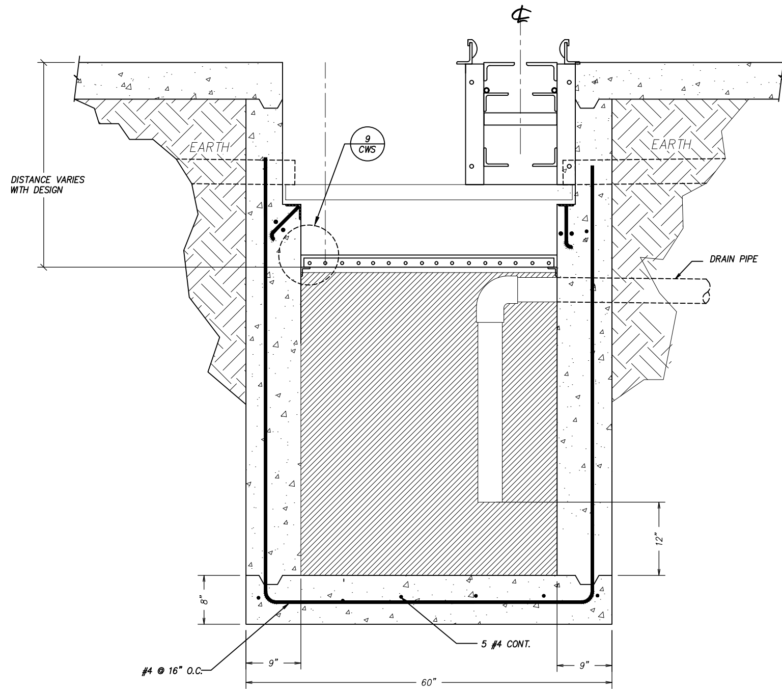
3 CWS SECTION THRU TRENCH
