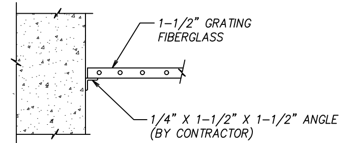
9 CWS BAR GRATE DETAIL
