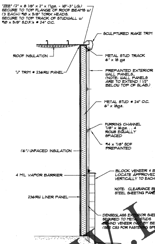
B SECTION AT EXTERIOR STUDWALL ENDWALL NOT TO SCALE
