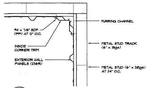
F INSIDE CORNER STUDWALL DETAIL NOT TO SCALE
