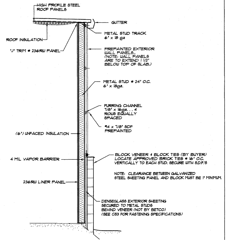
E SECTION AT EXTERIOR STUDWALL SIDEWALL NOT TO SCALE
