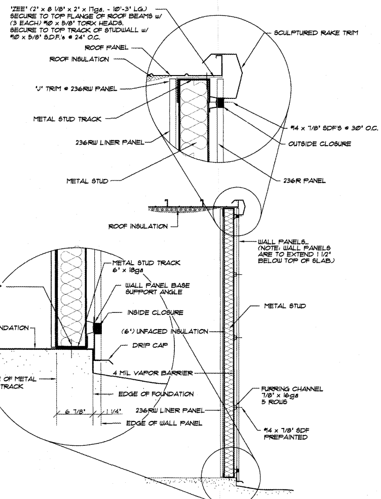
A SECTION AT EXTERIOR STUDWALL SIDEWALL NOT TO SCALE
