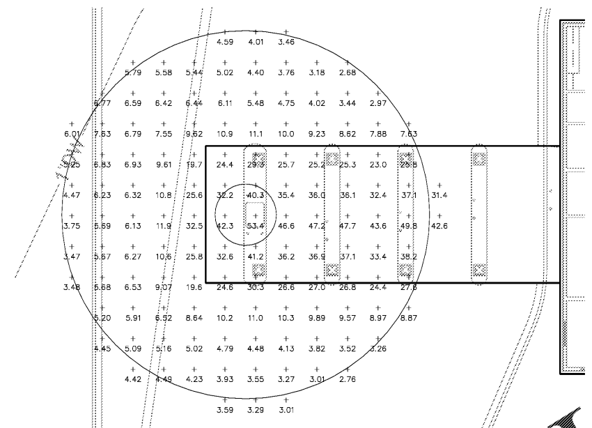
ATM - PHOTOMETRICS SCALE: 1" = 10'-0"
