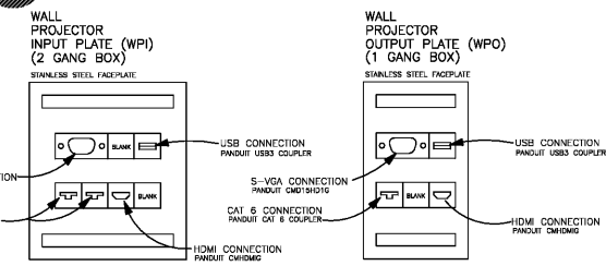
DETAIL - PROJECTOR PLATES N.T.S. (PROGRAM AREA 124)
