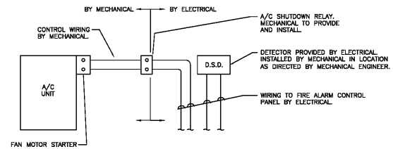
DETAIL - DUCT SMOKE DETECTOR CONNECTION N.T.S.
