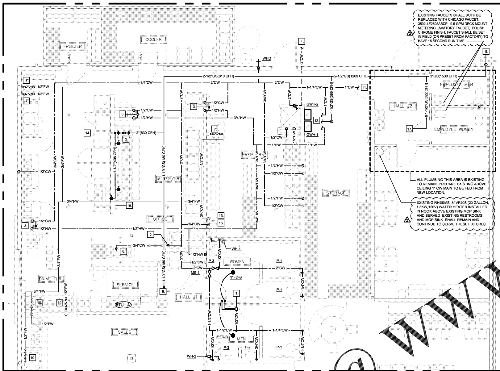
1 ENLARGED PLUMBING PLAN - WATER AND GAS PIPING SCALE: 1/4" = 1'-0"
