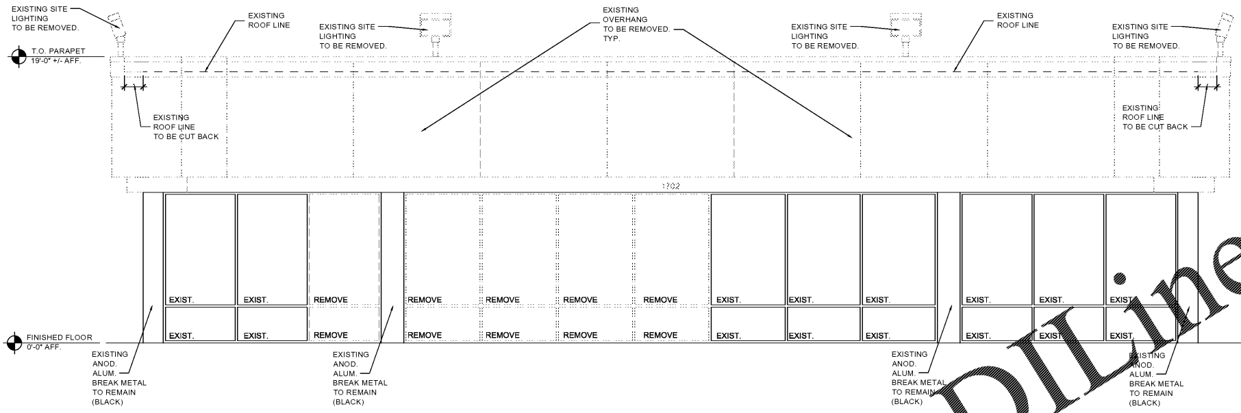
1 DEMOLITION FRONT ELEVATION D2 1/4"=1'-0"
