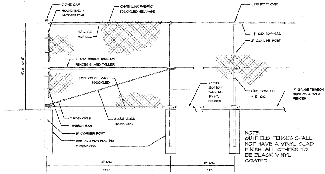
1 CHAINLINK FENCE - TYPICAL NOT TO SCALE
