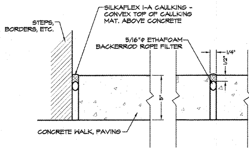
TYPICAL SECTION
