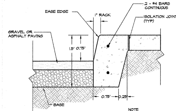
7 INTEGRAL CURB AT WALK NOT TO SCALE
