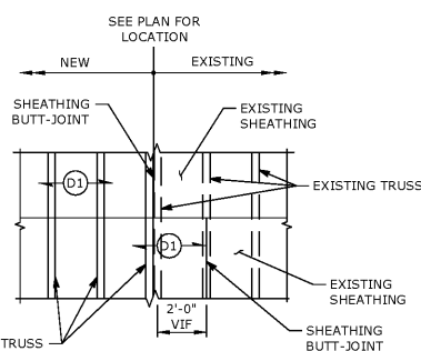
PARTIAL PLAN TYPICAL LAP DETAIL AT ROOF SHEATHING
