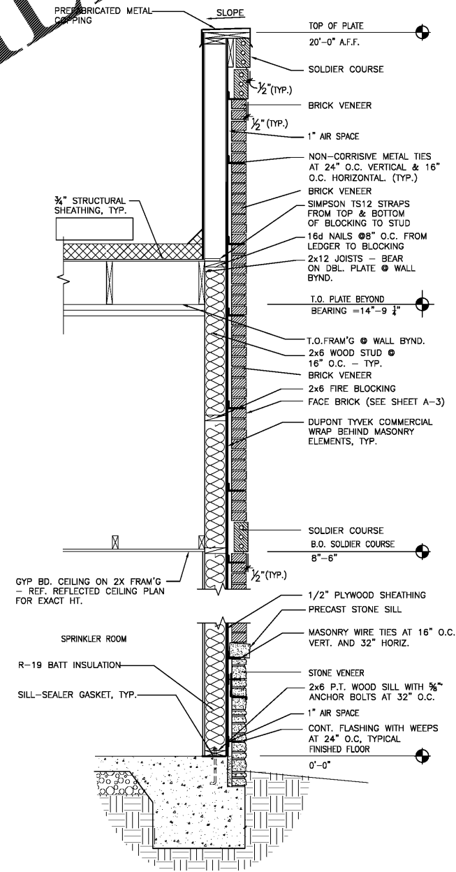
1 WALL SECTION • SPRINKLER RISER ROOM SCALE: 3/4" = 1'-0"
