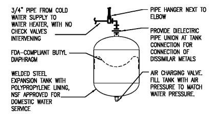
13 SMALL EXPANSION TANK NOT TO SCALE
