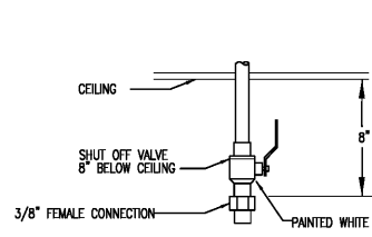
2 AIR DROP AT CEILING NOT TO SCALE
