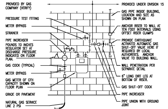
7 GAS METER SETTING NOT TO SCALE
