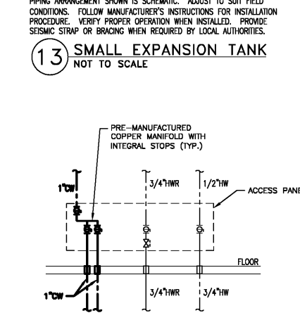
15 UPONOR MANIFOLD NOT TO SCALE
