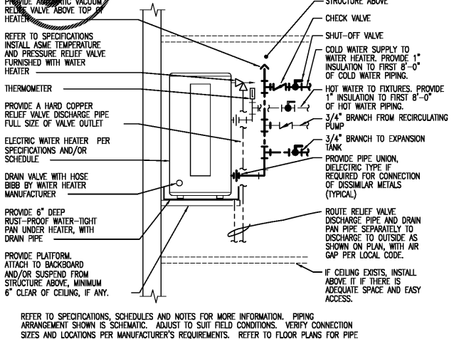
12 ELECTRIC WATER HEATER OVERHEAD NOT TO SCALE
