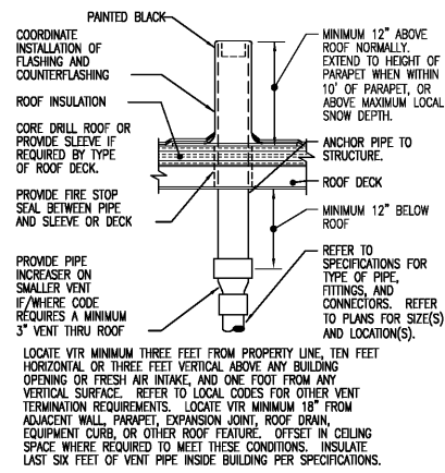
1 VENT THRU ROOF ("VTR") NOT TO SCALE
