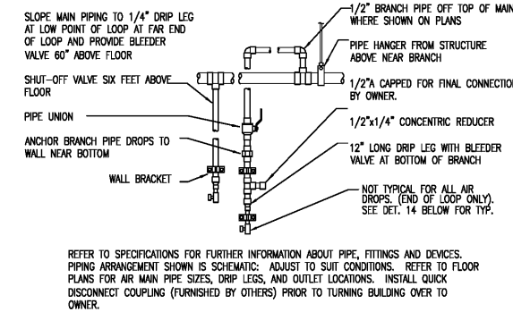
4 COMPRESSED AIR OUTLET NOT TO SCALE
