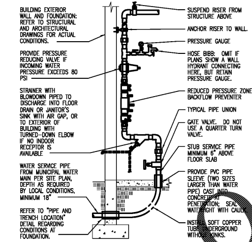
10 DOMESTIC WATER SERVICE ENTRY NOT TO SCALE
