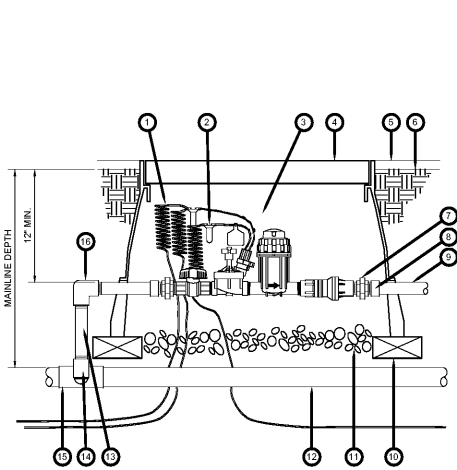
D DRIP CONTROL ZONE KIT SCALE: NTS
