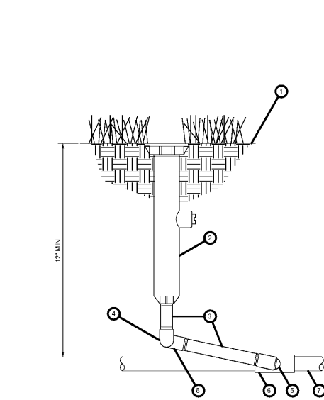
F POP-UP SPRAY HEAD SCALE: NTS
