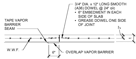
TYPICAL SLAB CONSTRUCTION JOINT w/ DOWELS 3/4" = 1'-0"
