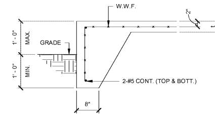
TYPICAL TURN-DOWN SLAB 3/4" = 1'-0"
