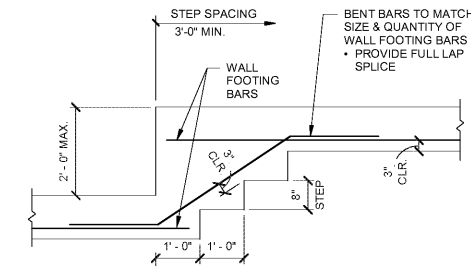
TYPICAL STEPPED FOOTING DETAIL 1/2" = 1'-0"
