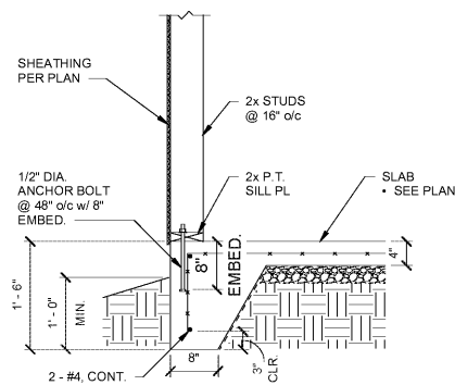
TURN DOWN SLAB w/ STUD WALL 3/4" = 1'-0"
