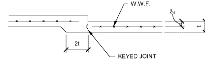
TYPICAL DEPRESSED SLAB-ON-GRADE 3/4" = 1'-0"
