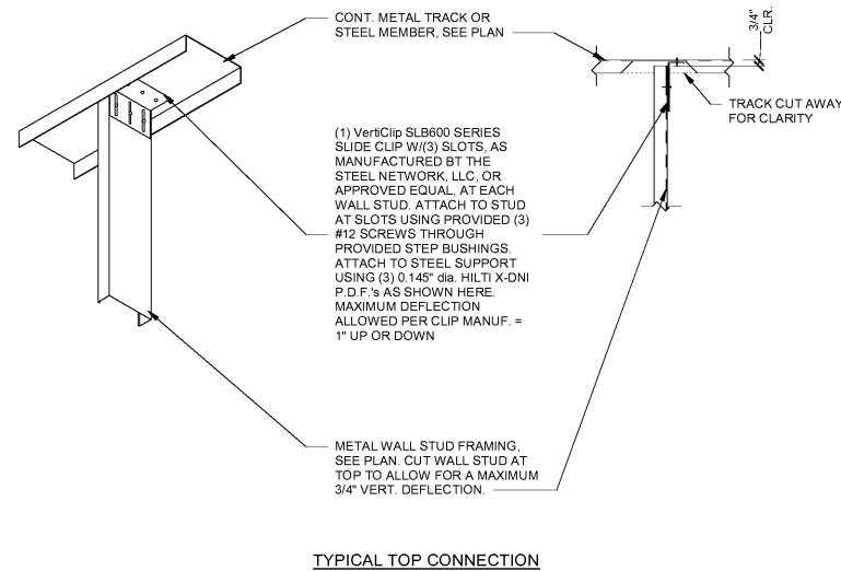
TYPICAL METAL STUD WALL SLIDE CLIP DETAILS 1" = 1'-0"
