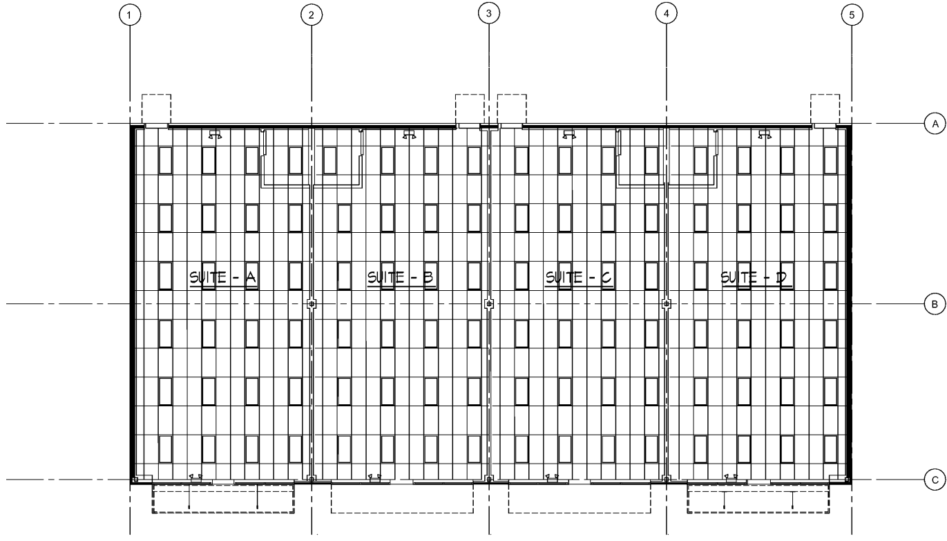
REFLECTED CEILING PLAN AT RETAIL/OFFICE SUITES SCALE: 1/8"=1'-0"
