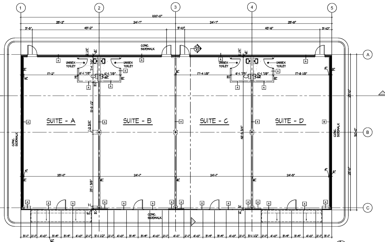
ARCHITECTURAL FLOOR PLAN - RETAIL/OFFICE SUITES
