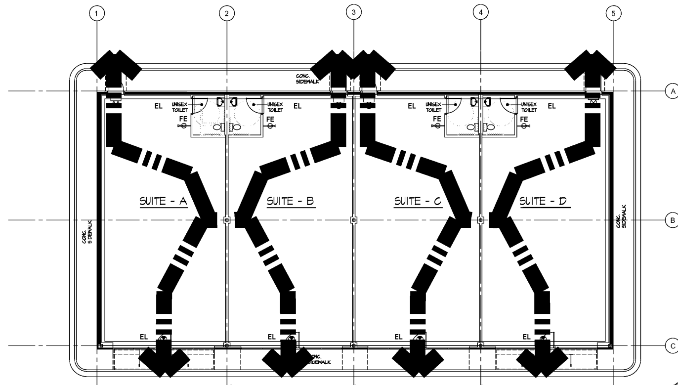
RETAIL/OFFICE SUITES - ACCESSIBILITY PLAN
