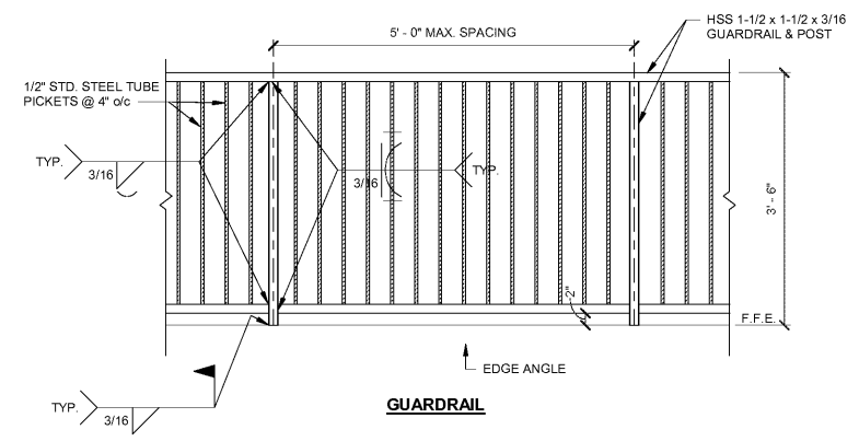
1 STAIR DETAIL 5302 3/4" = 1'-0"
