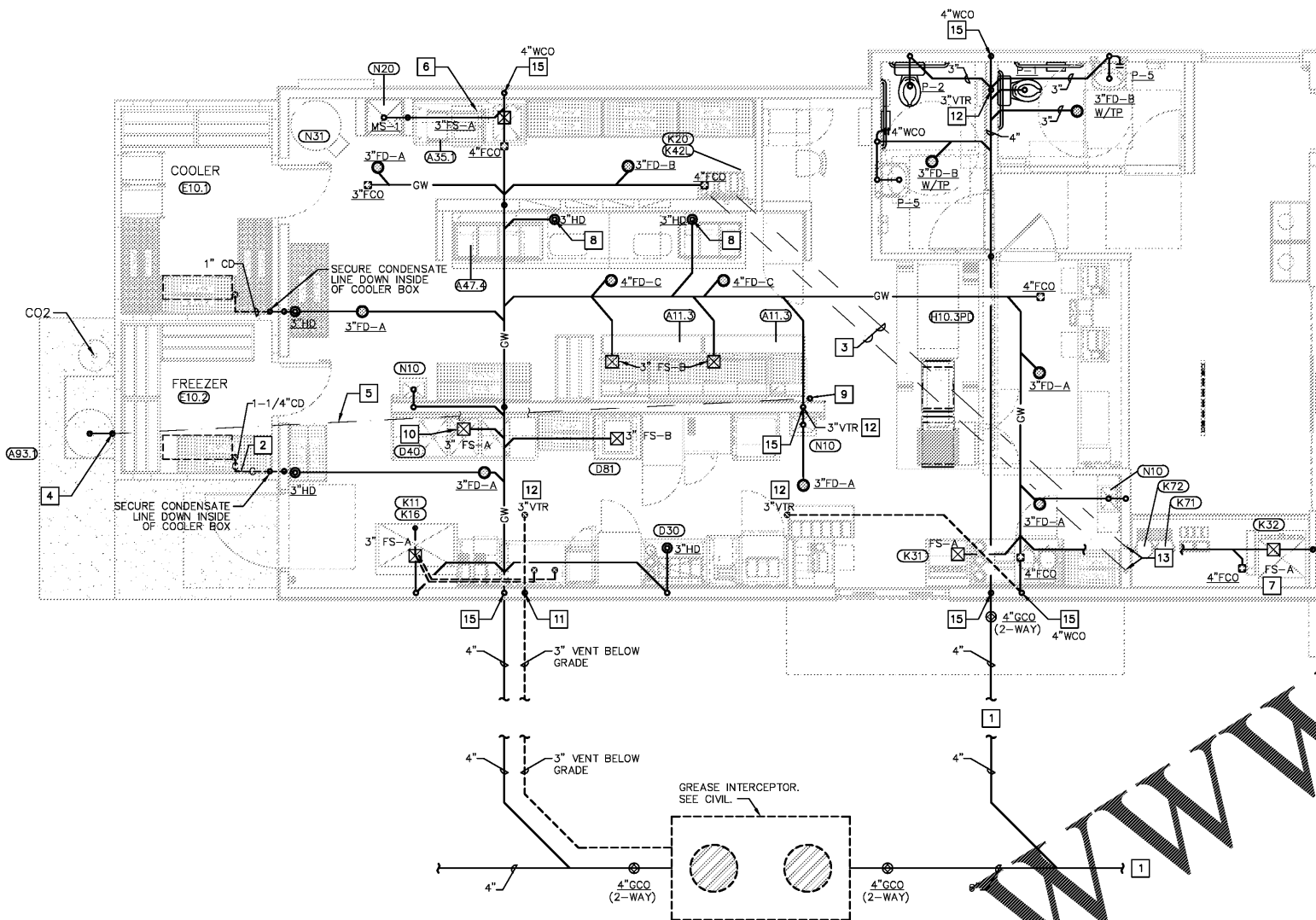
1 PLUMBING PLAN - WASTE & VENT PLAN 1/4" = 1'-0"
