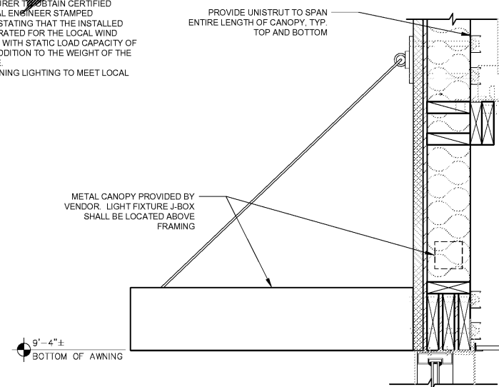
5 SECTION DETAIL - AWNING Scale: 1-1/2"=1'-0"
