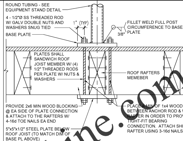
2 BASE PLATE CONNECTION DETAIL N.T.S.
