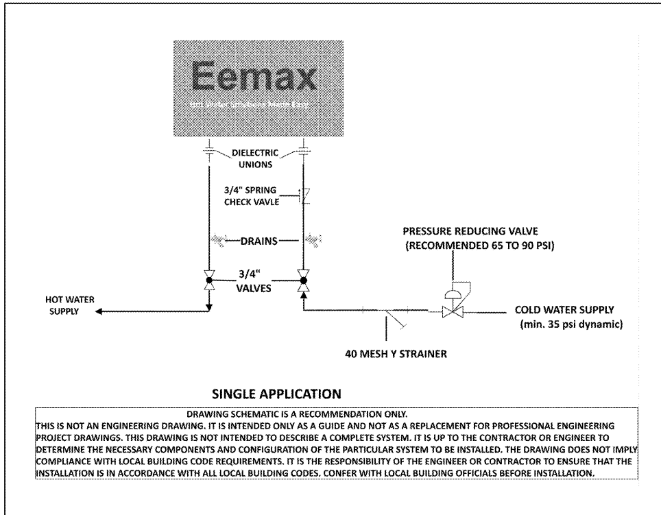
1 WATER HEATER 1 DETAIL SCALE NTS
