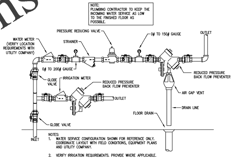
4 WATER SERVICE ENTRANCE DETAIL SCALE NTS
