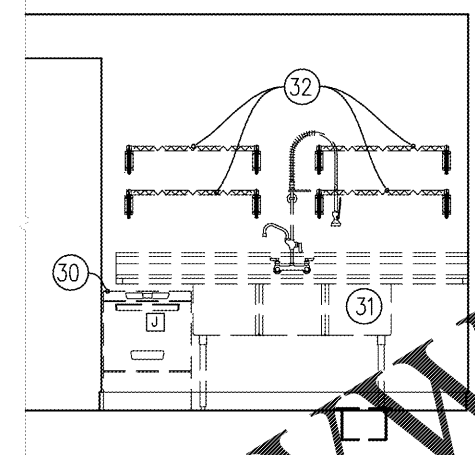
2 EQ-4 UTILITY 110 SCALE 1/2" = 1'-0"
