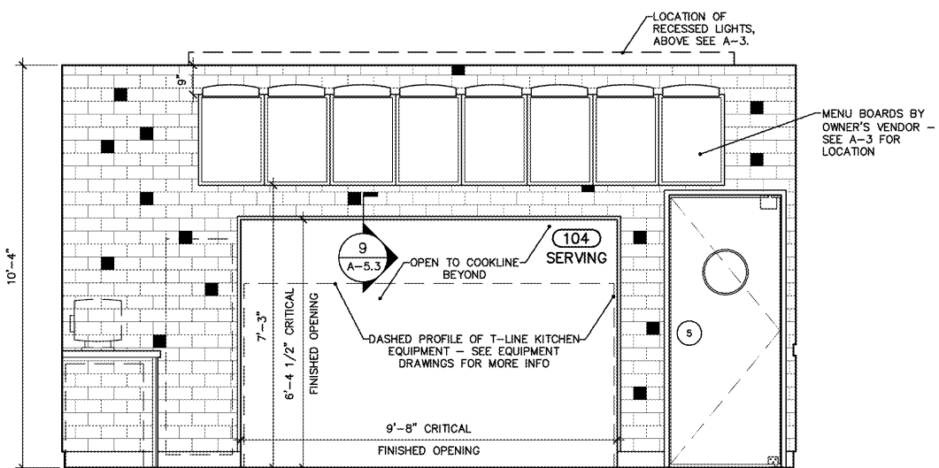
1 SERVICE COUNTER – MENU BOARD PLACEMENT A-8.2 SCALE 1/2" = 1'-0"
