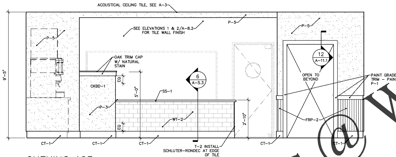
2 QUEUING 103 A-8.1 SCALE 1/2" = 1'-0"
