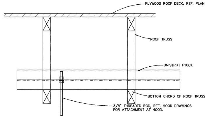
7 S-4 HOOD SUSPENSION DETAIL SCALE: 3" = 1'-0"
