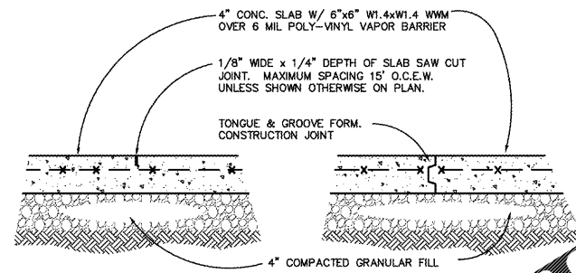
6 CONCRETE SLAB DETAIL SCALE: 1 1/2" = 1'-0"
