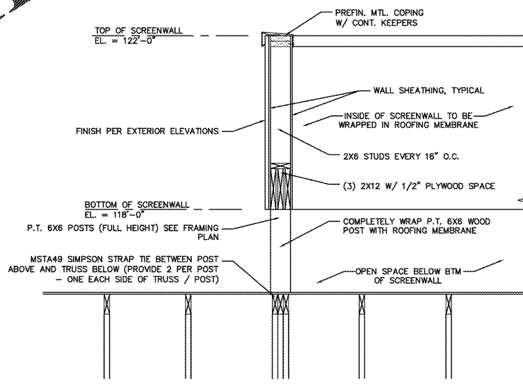
8 SCREENWALL FRAMING DETAIL SCALE: 3/4" = 1'-0"
