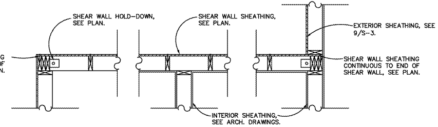
3 SHEAR WALL DETAIL SCALE: 3/4" = 1'-0"
