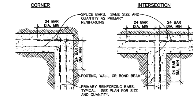
3 SHEAR WALL DETAIL SCALE: 3/4" = 1'-0"
