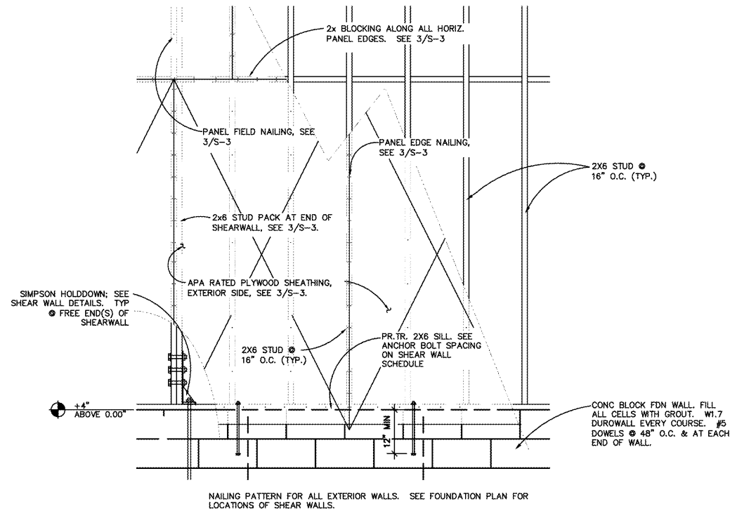
9 EXTERIOR WALL & SHEATHING/NAILER CONNECTION DETAIL SCALE: 3/4" = 1'-0"
