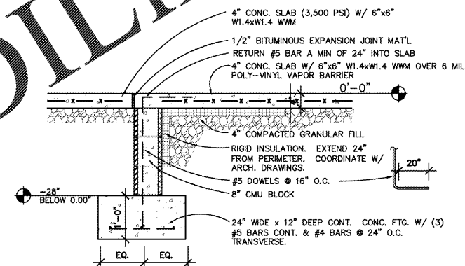
2 TURNED DOWN SLAB @ DOOR SCALE: 3/4" = 1'-0"
