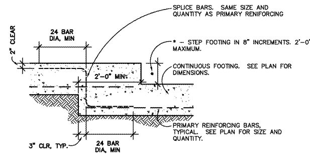
5 FOUNDATION STEP DETAIL SCALE: NONE
