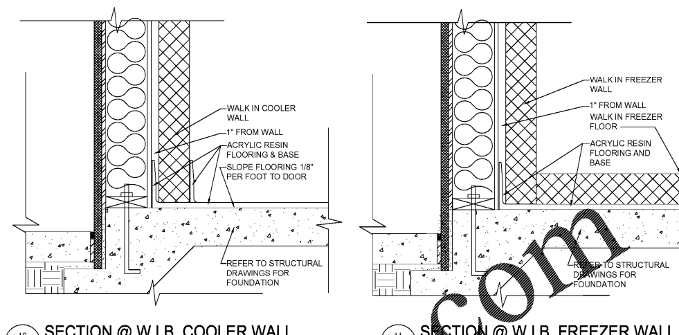
10 SECTION @ W.I.B. COOLER WALL
