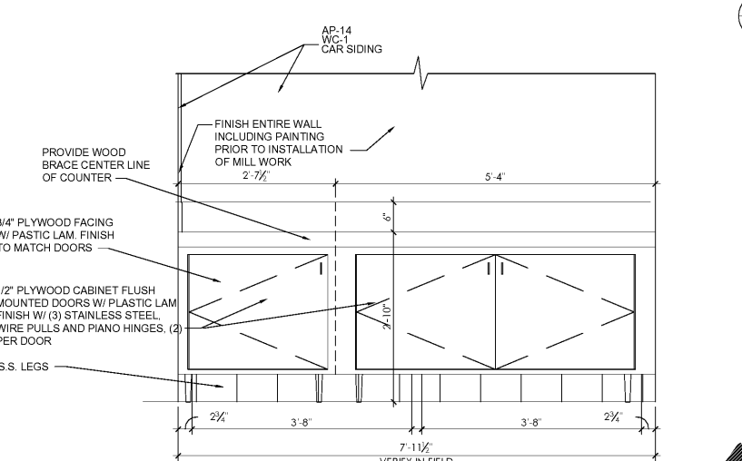
2 SELF-SERVE COUNTER ELEVATION
