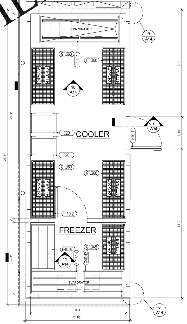
6 WALK IN FLOOR PLAN
