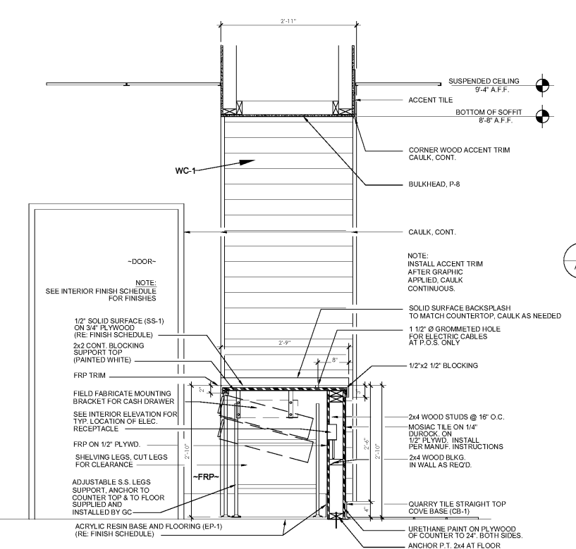
1 SECTION @ FRONT COUNTER
