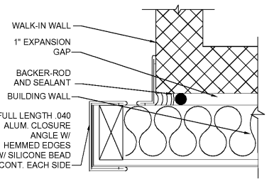
9 FLASHING DETAIL @ W.I.B.
