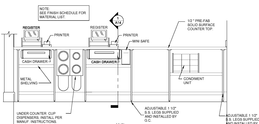
5 FRONT COUNTER REAR ELEVATION
