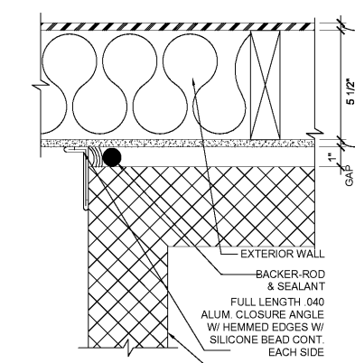
8 FLASHING DETAIL @ W.I.B.
