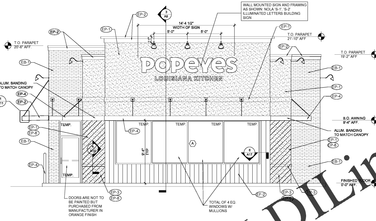
1 FRONT ELEVATION
