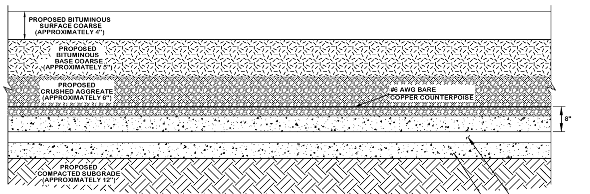
SECTION L-852G IN-PAVEMENT RUNWAY GUARD LIGHT INSTALLATION IN NEW BITUMINOUS PAVEMENT - STEP 1
