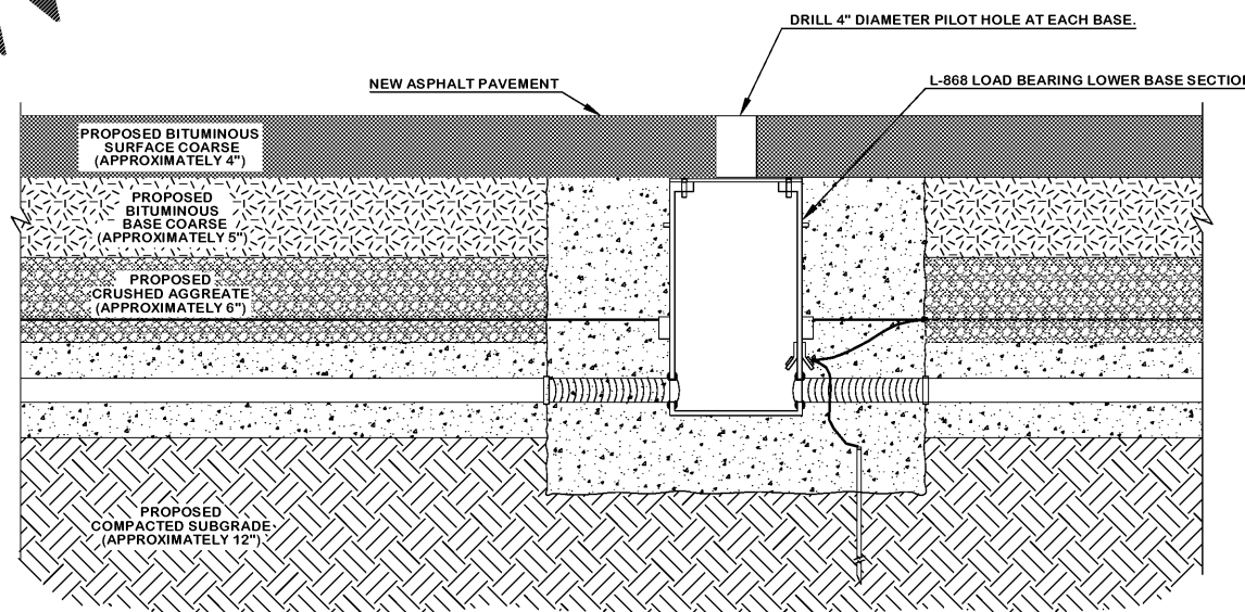
SECTION L-852G IN-PAVEMENT RUNWAY GUARD LIGHT INSTALLATION IN NEW BITUMINOUS PAVEMENT - STEP 4
