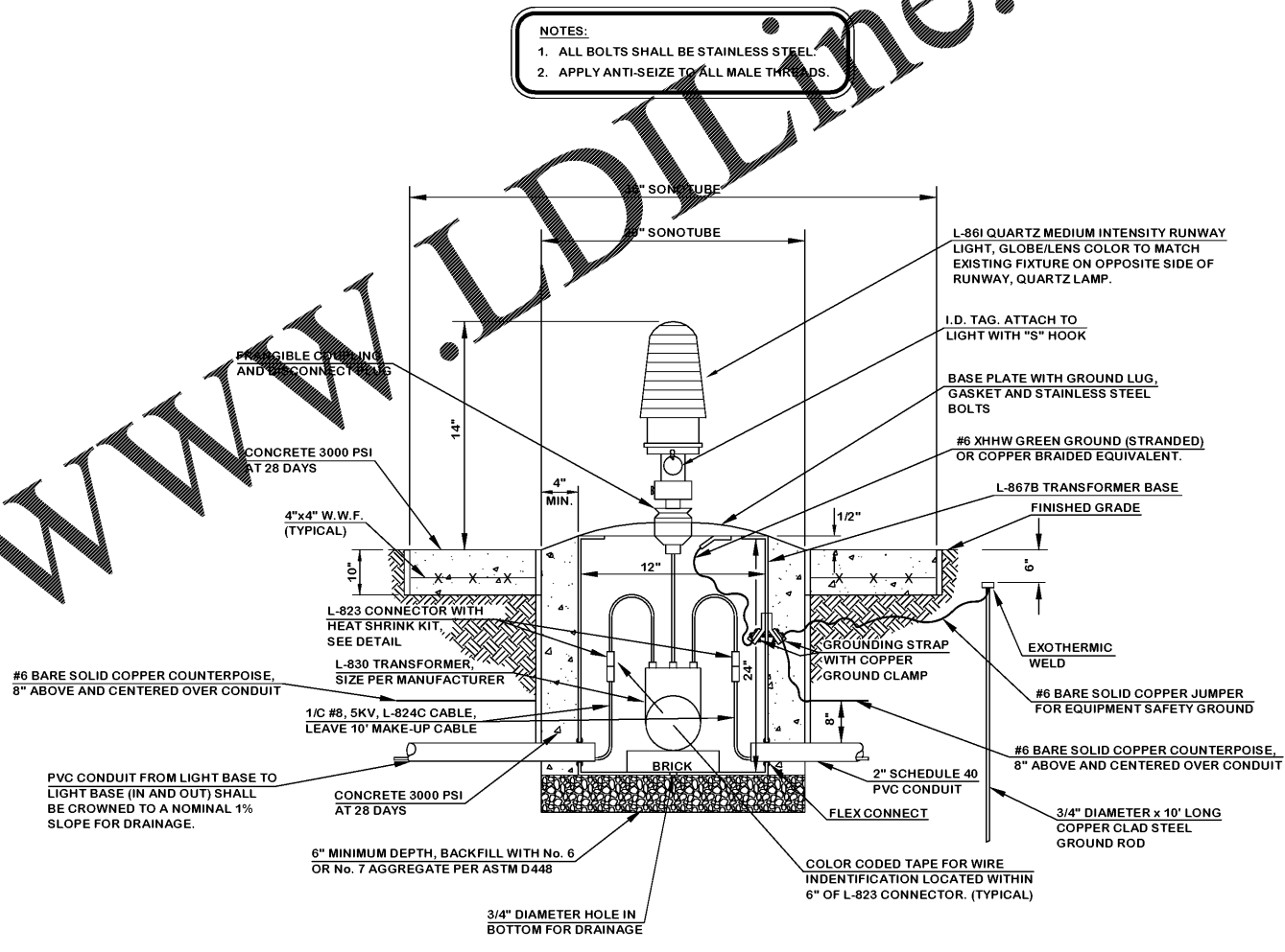
SECTION BASE MOUNTED MEDIUM INTENSITY RUNWAY LIGHT IN TURF SHOULDER DETAIL N.T.S.
