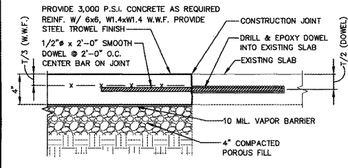
SLAB JOINT DETAIL
