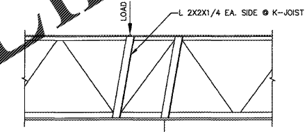
JOIST CONCENTRATED LOAD REINFORCEMENT
