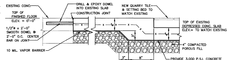
DEPRESSED SLAB JOINT DETAIL
