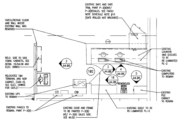
1 REMODELED WORK ROOM DETAIL PLAN A4.06 SCALE: 1/4" = 1'-0"
