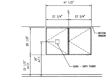
19 COMMUNICATION CABINET INSTALLATION DETAIL A4.06 N.T.S.
