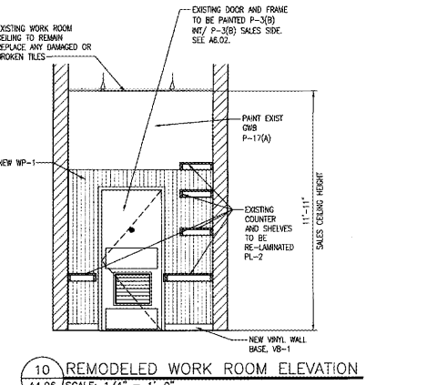
10 REMODELED WORK ROOM ELEVATION A4.06 SCALE: 1/4" = 1'-0"
