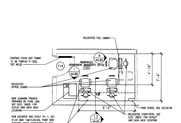
6 REMODELED DEPT. MANAGERS OFFICE DETAIL PLAN A4.06 SCALE: 1/4" = 1'-0"
