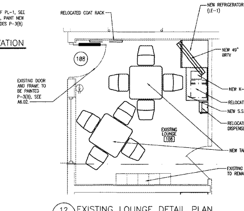
12 EXISTING LOUNGE DETAIL PLAN A4.06 SCALE: 1/4" = 1'-0"
