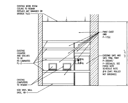
4 REMODELED WORK ROOM ELEVATION A4.06 SCALE: 1/4" = 1'-0"
