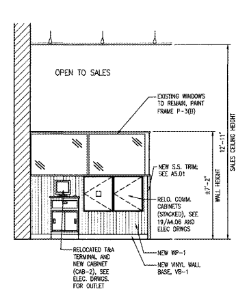
2 REMODELED WORK ROOM ELEVATION A4.06 SCALE: 1/4" = 1'-0"
