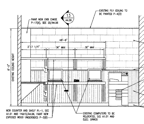
7 REMODELED DEPT. MGR. OFFICE ELEVATION A4.06 SCALE: 3/8" = 1'-0"
