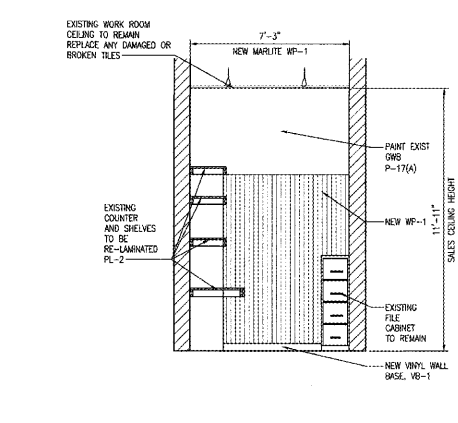
3 REMODELED WORK ROOM ELEVATION A4.06 SCALE: 1/4" = 1'-0"
