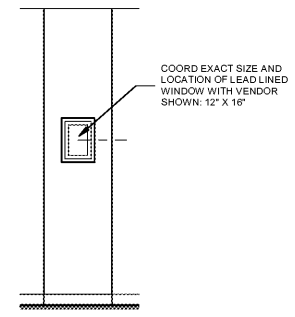
12 X-RAY WINDOW ELEV 3/8" = 1'-0"
