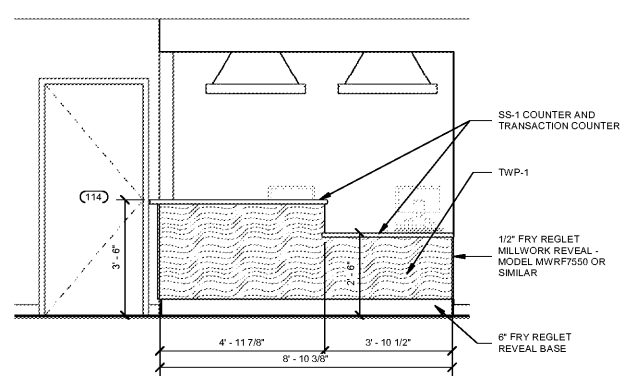
1 WAITING ROOM FRONT ELEV 3/8" = 1'-0"
