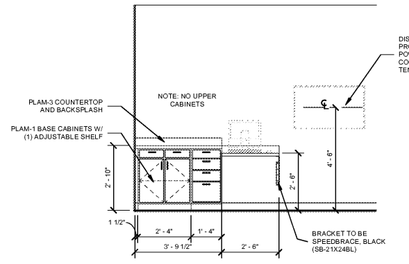
8 LARGE EXAM ROOM ELEV 3/8" = 1'-0"
