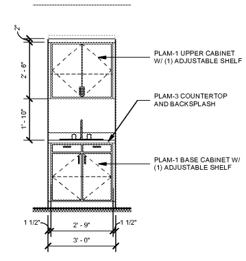
5 TYPICAL HALL HANDWASH STATION 3/8" = 1'-0"
