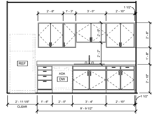
13 BREAK ROOM 139 ELEV 3/8" = 1'-0"
