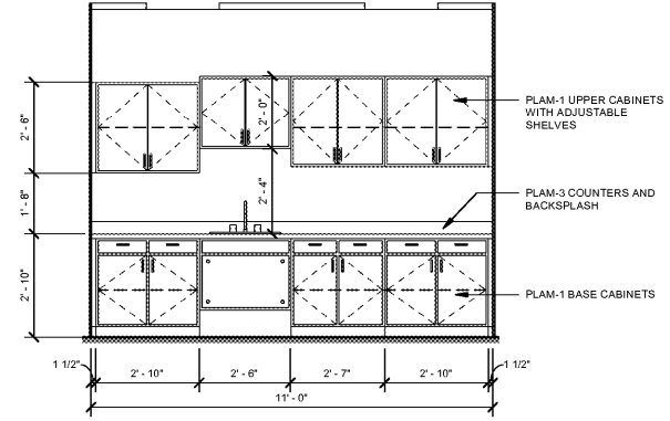
10 CAST 117 ELEV 3/8" = 1'-0"
