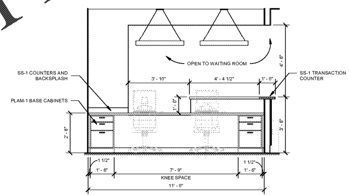
3 RECEPTION 115 ELEV 3/8" = 1'-0"
