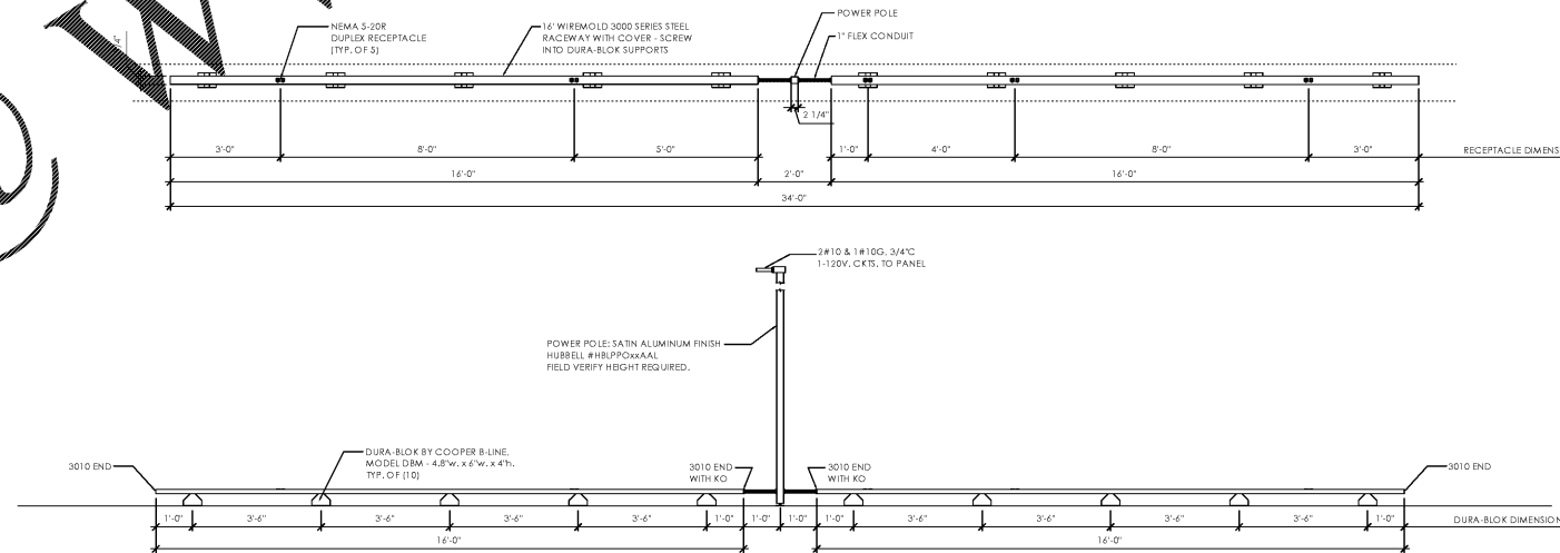
Gondola Lighting Raceway Detail
