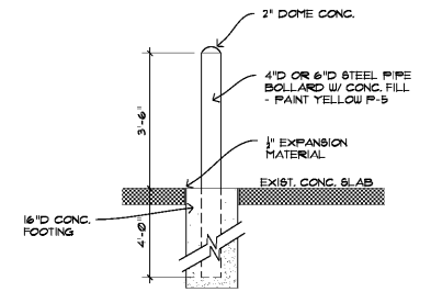
5 STEEL PIPE BOLLARD DETAIL 1/2" = 1'-0"
