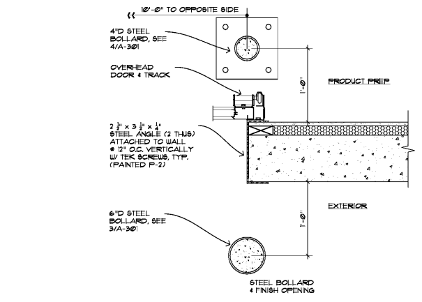
6 OH. DOOR JAMB DETAIL 1/2" = 1'-0"
