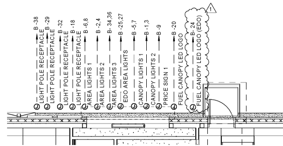
3 TYPICAL SITE LIGHTING CIRCUITS 3/16" = 1'-0"
