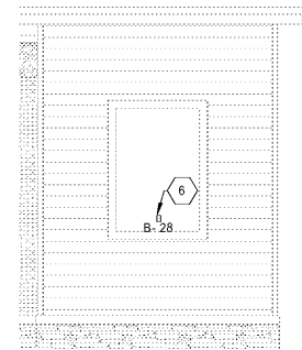
2 CORNER TOWER FRONT ELEVATION 3/16" = 1'-0"
