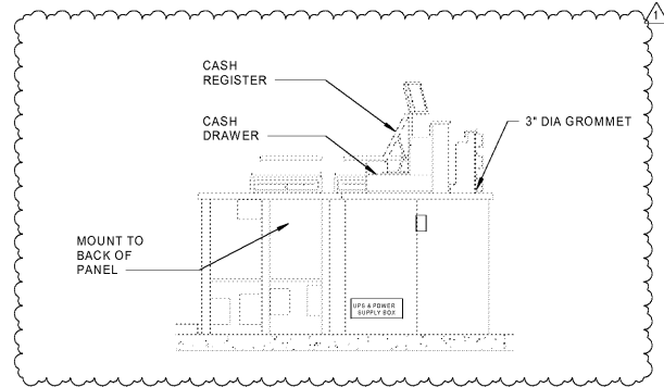
3 CASHWRAP SECTION 1/2" = 1'-0"
