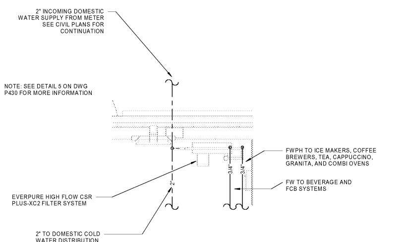
2 ENLARGED WATER PLAN 1/2" = 1'-0"
