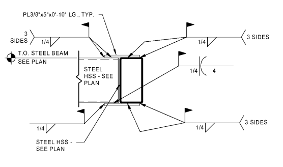
3 HSS TO HSS BEAM CONNECTION 3/4" = 1'-0"
