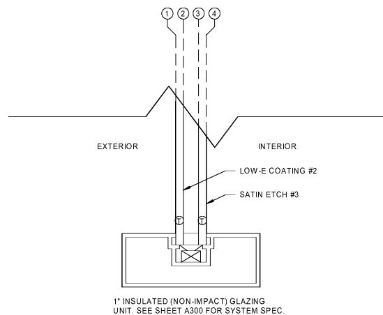
6 NON-IMPACT RATED SYSTEM 6\"/>
