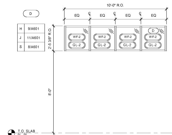
1 STOREFRONT ELEVATION D 3/8\"/>
