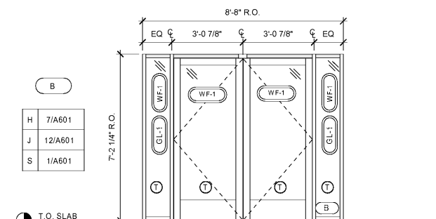
2 STOREFRONT ELEVATION B 3/8\"/>
