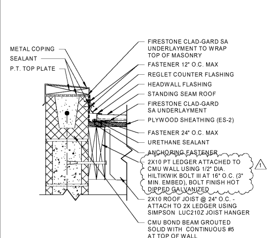
9 SECTION DETAIL 1 1/2" = 1'-0"
