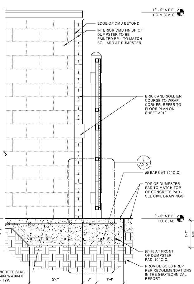
2 DUMPSTER FRONT WALL 3/4" = 1'-0"
