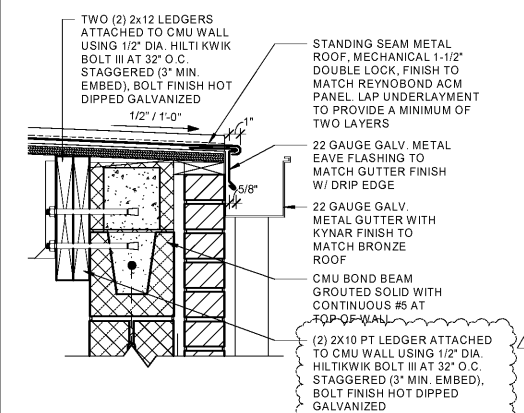
8 SECTION DETAIL 1 1/2" = 1'-0"
