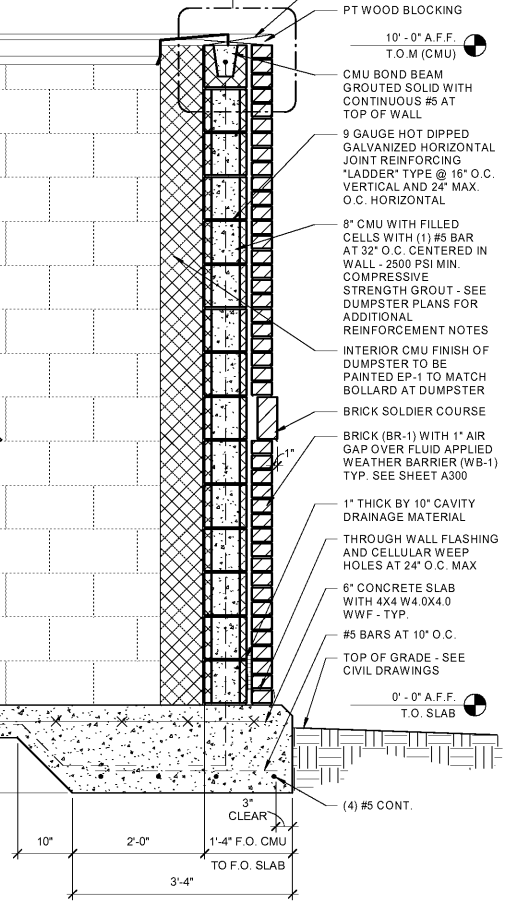
1 DUMPSTER SIDE WALL 3/4" = 1'-0"
