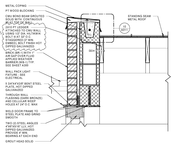
7 SECTION DETAIL 1 1/2" = 1'-0"
