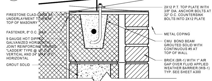
6 SECTION DETAIL 3" = 1'-0"
